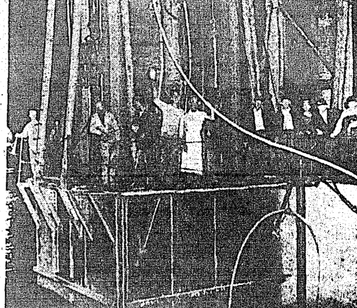
RADAR DEFENSE . . . Platform of 6,200 ton "Texas Tower" type radar station is towed from Portland, Maine, to Nantucket, Mass., for installation.
