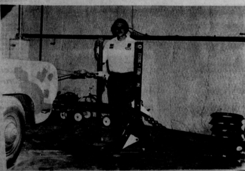
PICTURED ABOVE IS THE BODY SHOP MANAGER, DARL HERGERT, WITH THE KANSAS JACK "POWER POST". THIS MACHINE DELIVERS UP TO 20 TONS OF FORCE TO DAMAGED STEEL AND SHEET METAL. THIS IS JUST ONE PIECE OF MODERN EQUIPMENT DARL USES TO MAKE SURE YOUR AUTO BODY REPAIRS ARE OF THE HIGHEST QUALITY. FOR THE BEST BODY, PAINT AND GLASS SERVICE YOUR MONEY CAN BUY, CALL ON DARL.
