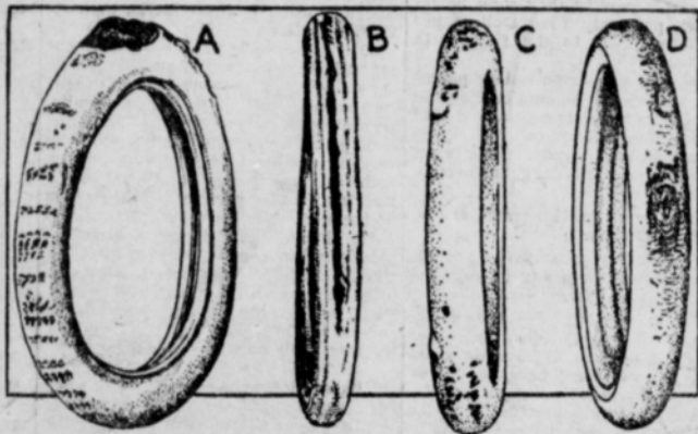
Some Common Abuses of Tires—A Shows the Result of Improperly Fitted Tire Chains—B, Faulty Wheel Alignment—C, Neglected Cuts, and D, Results of Skidding.
