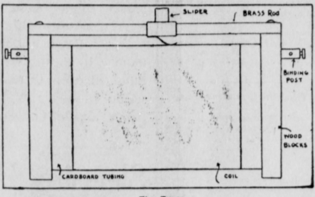
The Tuner.
