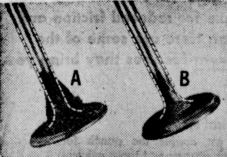
"Coked" valve "A" is from engine using so-called "all-season," multi-grade oil. Coke-like carbon deposit is a cause of sluggish performance and ultimate valve failure. Clean valve "B" is from engine using new Gulfpride.
