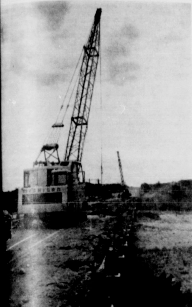
DEATH OF A BRIDGE —Two giant power hammers are shown above beating out the reinforced concrete floor in Quit- River Bridge on State Highway 70, northeast of Flomot. A new and wider bridge will replace the structure which was damaged several years ago by floods. Most of the steel will be salvaged from the old bridge. Paved detour crossing is pro- vided for traffic while the old bridge is being replaced.
