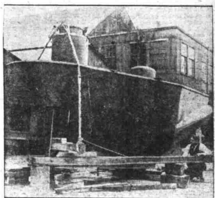
Associated Press Photo This is Simon Lake's new submarine as it was prepared for shipment from Lancaster, Pa., to Bridgeport, Conn. It measures 22 feet in length. Lake, inventor of the even keel submarine, said the craft would be used for heretofore unattempted adventures. It is fitted with wheels to make progress on the sea bottom possible.
