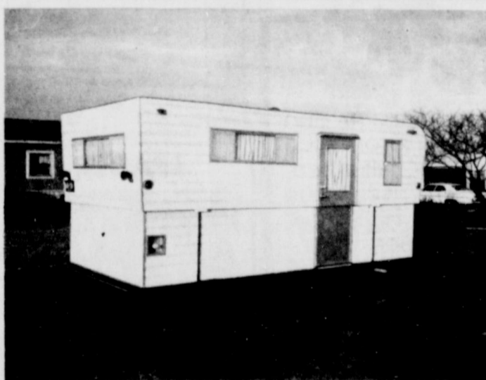
THIS self-contained camper was completely constructed locally by Billy Craig, Tahoka electrician. A hydraulic system lowers the top half to car top level for efficient roadability.
