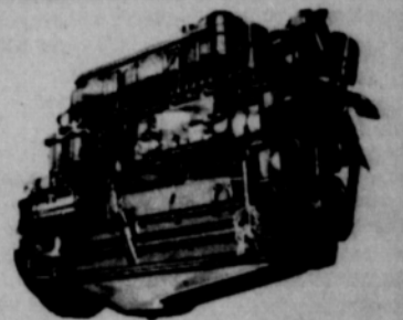
Massive engine—Brawny, 6 cylinder moderate speed engine has heavily ribbed block, multiple cylinder heads. Seven bearing crankshaft. 15-inch clutch. Diesel engine is 401 cubic inch; gasoline and LP-gas are 377 cubic inch.
