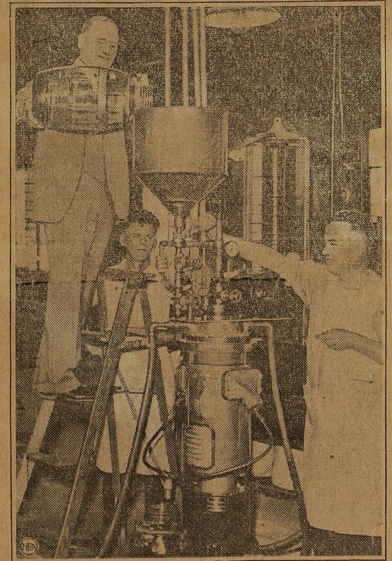
Whisky aged while you wait! That's the claim made for this high voltage machine. One of the inventors, W. A. Morgan, is shown pouring raw liquor into the apparatus at a demonstration in Buffalo, N. Y.
