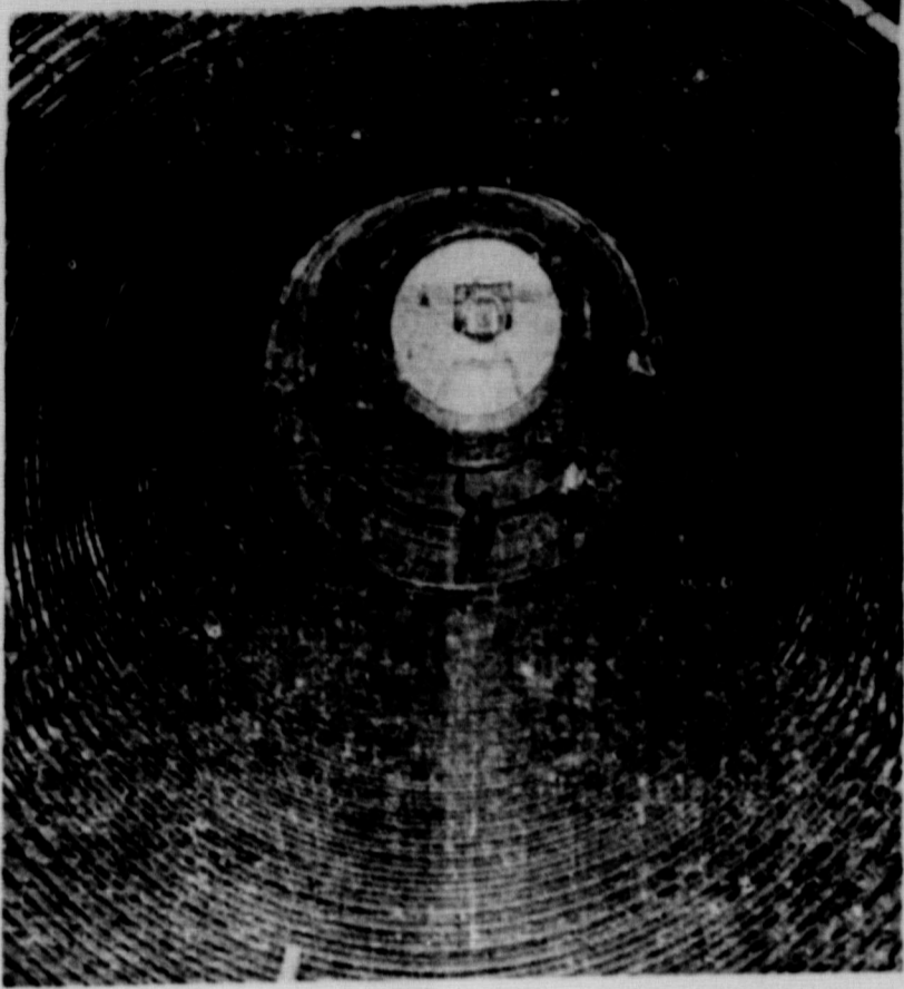
COLUMBIA BASIN SIPHON... Near Adrian, Wash., steel workers weave web of heavy reinforcing bars around which will be poured concrete for Crab creek inverted siphon which will convey Columbia basin irrigation water across Dry Coulee to reclaim eastern Washington sagebrush land. Twenty-five feet in diameter and 4,500 feet long, it will be world's largest monolithic concrete pipeline.
