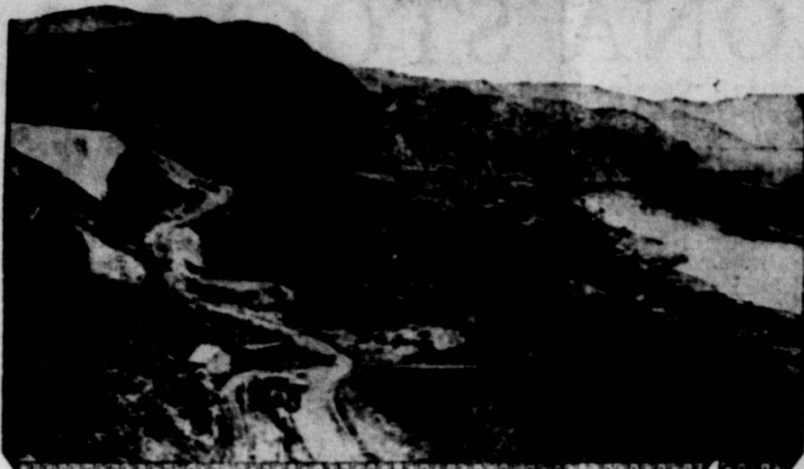
Aerial view of the Columbia River basin near Alder, Alaska, showing the site of the proposed Grand Coulee dam. The plans call for a dam 247 feet high and a power plant with eight generating units and an installed capacity of 700,000 horsepower. The I.W.A. has allotted about $10,000,000 for the project.
