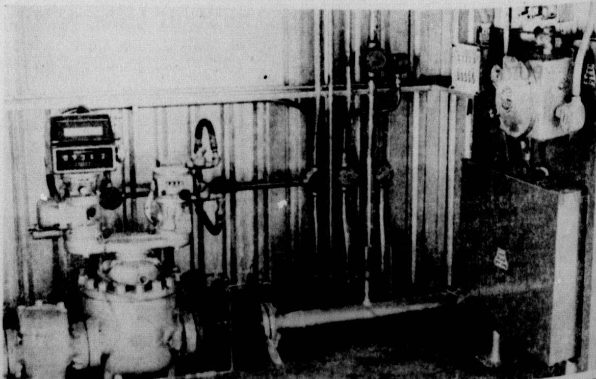
HELP YOURSELF meter and control equipment, shown here, permits driver-attended loading of LPG production. Numerous shutdowns are provided to assure a safe loading operation.
