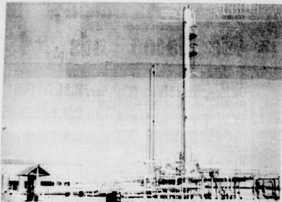
AN OVERALL VIEW of the process area shows the deethanizer and debutanizer fractionating columns with their accessory exchangers, pumps and vessels, the compressor building, left background and the electrical switchgear, left.
