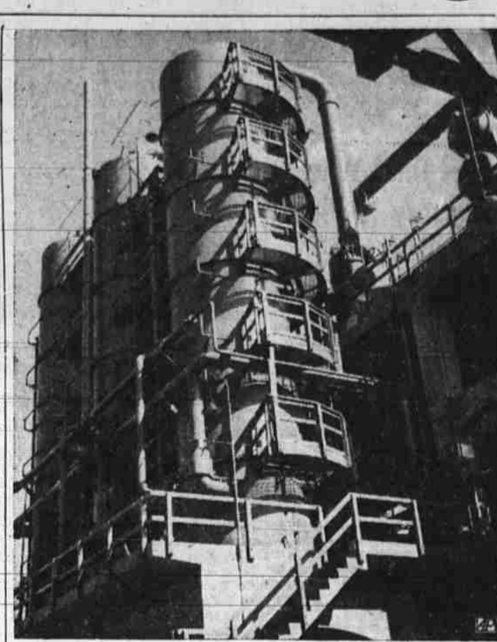
New Rubber Plant—These towers are a part of the new 60,000-ton synthetic rubber plant which will be opened at Houston formally Nov. 17.
