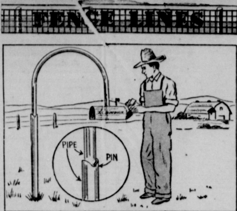
ROAD-MAINTENANCE MACHINERY WON'T TIP OVER this swinging mailbox. If a machine strikes the box, it swings out of the way, then swings back into position when machine has passed. Support stands back from road; box swings near road.
